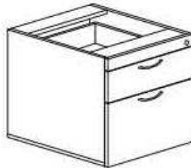
HANGING PEDESTAL 2D FO - H2 393W x 461D x 478H
